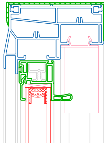
HEAD EXPANDER ON SERIES 500 DOUBLE HUNG
