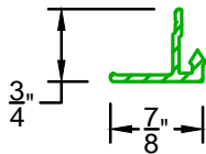
J TRIM FOR SERIES 300
