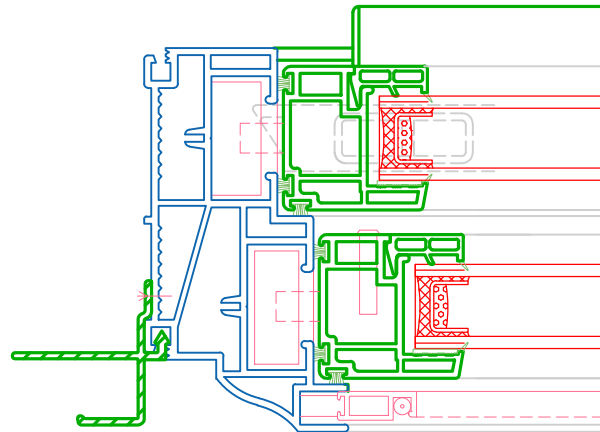
J TRIM WITH NAILING FIN ON SERIES 200 DOUBLE HUNG
