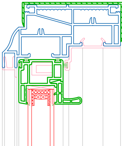
HEAD EXPANDER ON SERIES 200 DOUBLE HUNG
