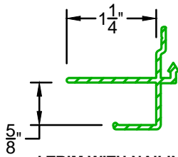
J TRIM WITH NAILING FIN FOR SERIES 200 & 500
