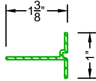
NAILING FIN FOR SERIES 100, 200 & 500
