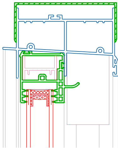
HEAD EXPANDER ON SERIES 100 DOUBLE HUNG
