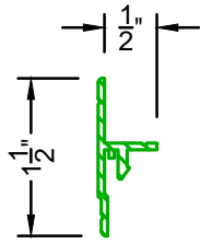
WOOD JAMB EXTENSION FOR SERIES 300 & 400
