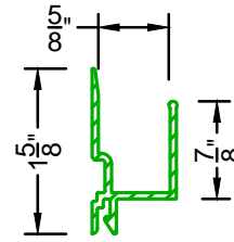
DRYWALL RETURN FOR SERIES 200, 300 & 400
