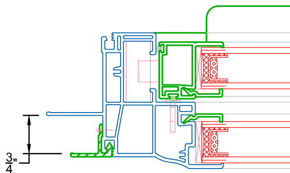
J TRIM ON SERIES 300 DOUBLE HUNG
